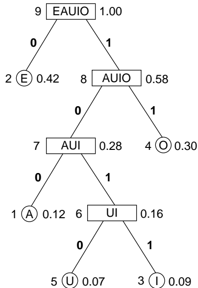
Figure 20.4.1. Huffman code for the fictitious language Vowelish, in tree form. A letter (A, E, I, O, or U) is encoded or decoded by traversing the tree from the top down; the code is the sequence of 0's and 1's on the branches. The value to the right of each node is its probability; to the left, its node number in the accompanying table.
